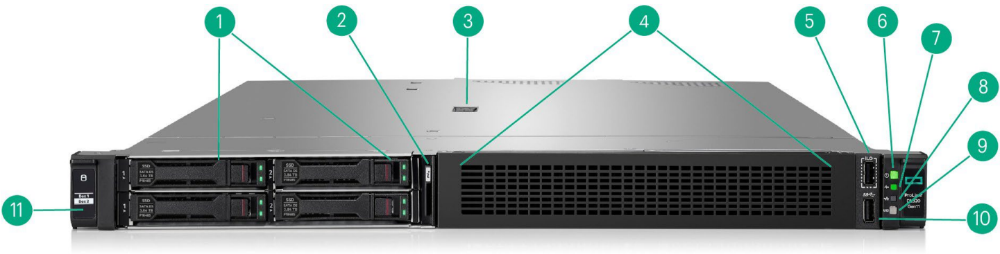
Front View – GPU CTO Server
