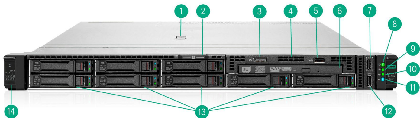
8SFF Front View - 8 SFF + optional Universal Media Bay, optical Drive, Display Port, USB 2.0, and SATA Drive shown
